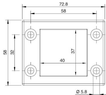
开孔尺寸 Platemounting dimensions
