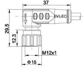
插孔 Female 90°
