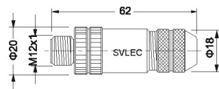
现场接线 / 螺钉压接 Field-wireable / screw terminals
