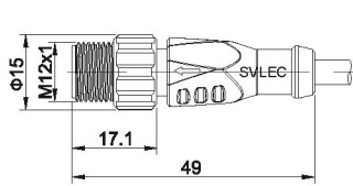
单端预铸线束 With open ended wires
