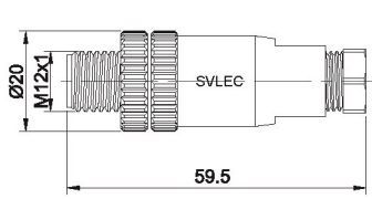
单端预铸线束 With open ended wires
