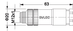
现场接线 / 可接 2 根电缆 Field-wireable / Can receive 2 cables can receive 2 cables
