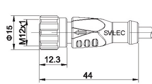
插孔 Female 直出 Straight
