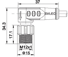
插针 Male 90°
