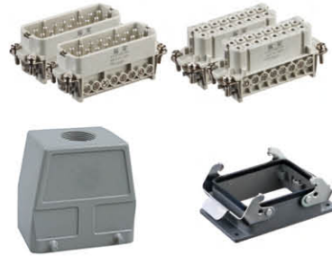
开孔顶出 Top-entry & bulkhead
