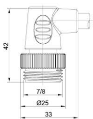
插针 Male 90°
