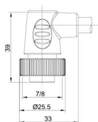
插孔 Female 90°
